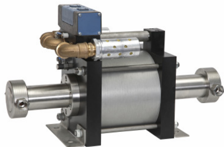
GPD120 double acting, single air drive head
